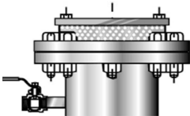
STANDARD EXIT ORIFICES ARE PROTECTED WITH PERFORATED ROUND HOLE STAINLESS SHEETING.
