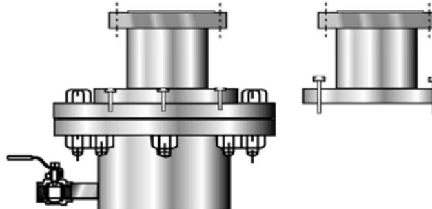
OPTIONAL ACCESSORY: REMOVE STANDARD SCREENING AND ADD RETROFIT SWIVEL FLANGED OUTLET. ALLAN HEAD CONNECTION.
