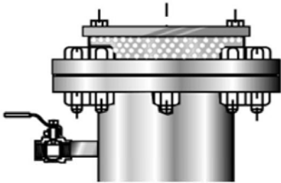
STANDARD EXIT ORIFICES ARE PROTECTED WITH PERFORATED ROUND HOLE STAINLESS SHEETING. FEMALE NPT THREAD CONNECTION
